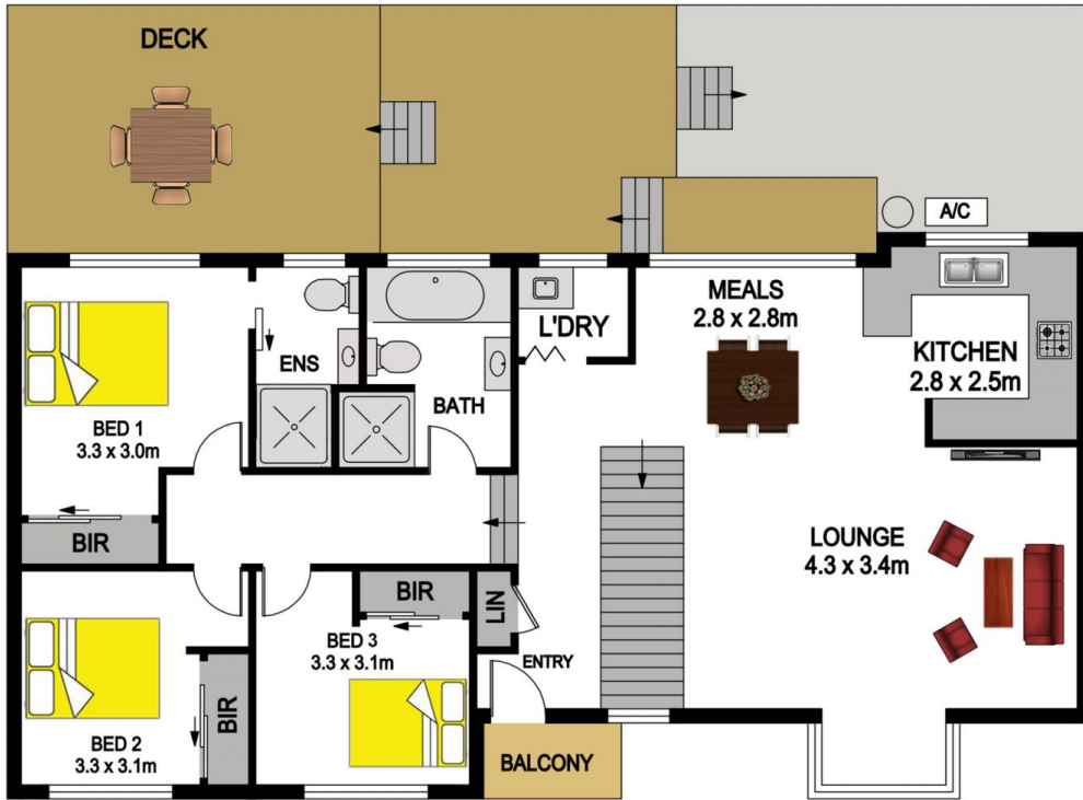
UPPER FLOOR
